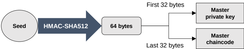
Figure B Master private key calculation from seed
